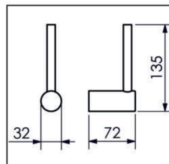
02.SG00.CR PAPELEIRA RESERVA
